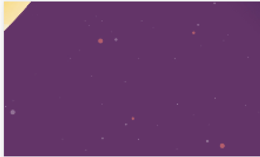
Patterns of Earth and Sky
