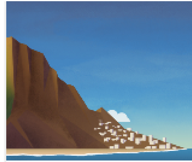
The Earth System
